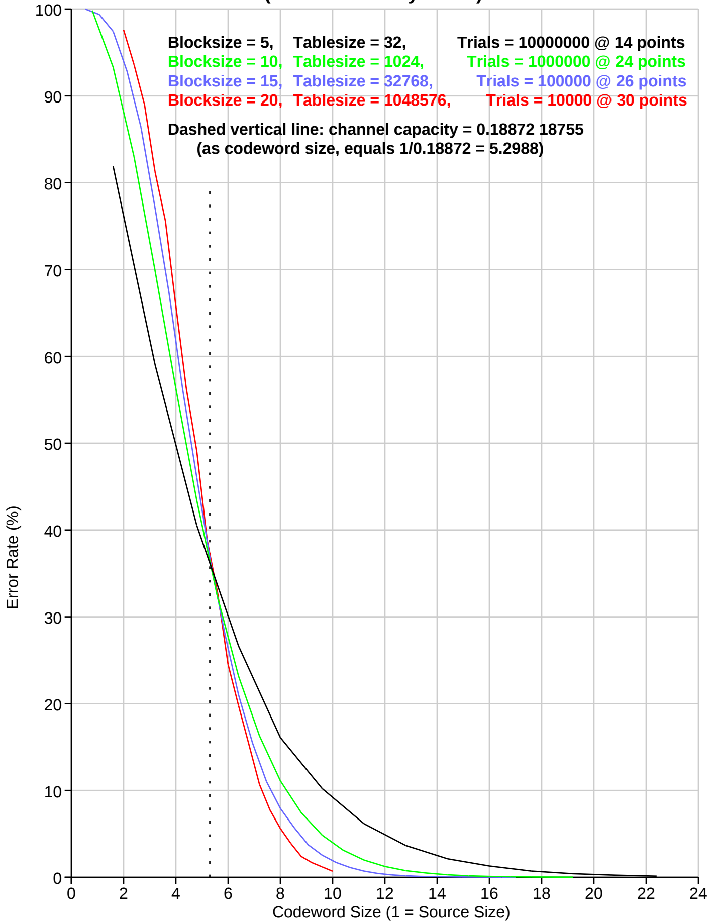
Figure 4.1 Simulation of Shannon's Random Codes
