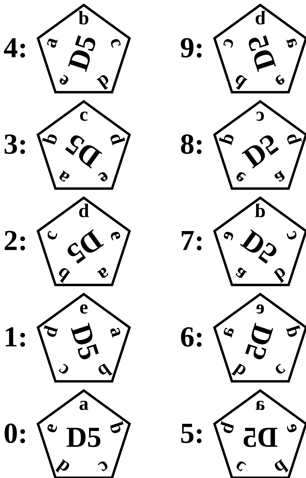
Figure 8.1 Elements of D_5 : Symmetries of a Pentagon.
